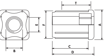
LONG THREADED SQUARE TUBE END
