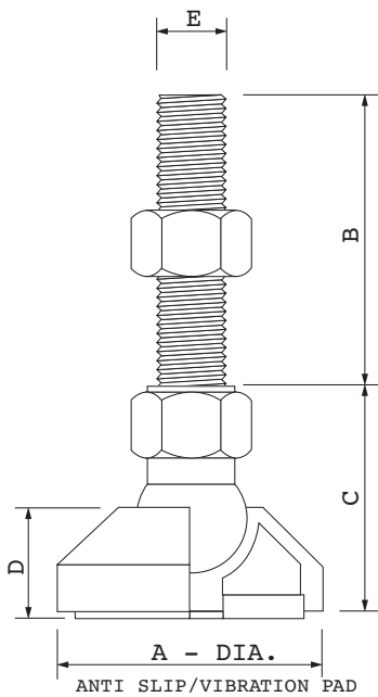
Ball Jointed A-justa-foot
