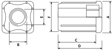
SQUARE THREADED TUBE END + SQUARE PLUG
